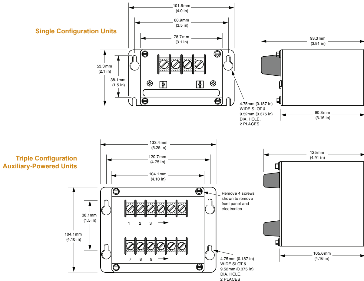
Figure 5. Outline Dimensions.
