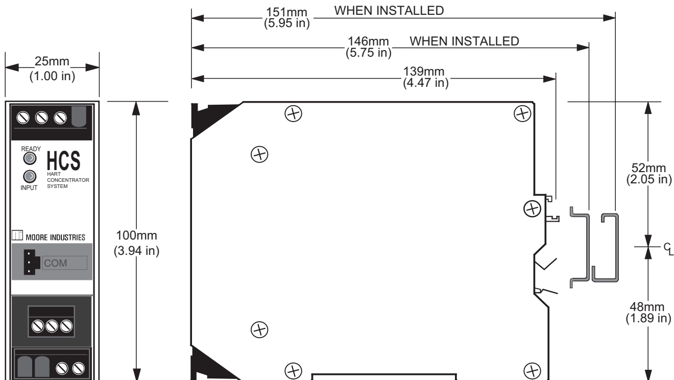
Figure 4. Installation Dimensions
