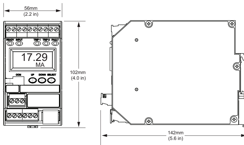
Figure 9. Installation Dimensions
