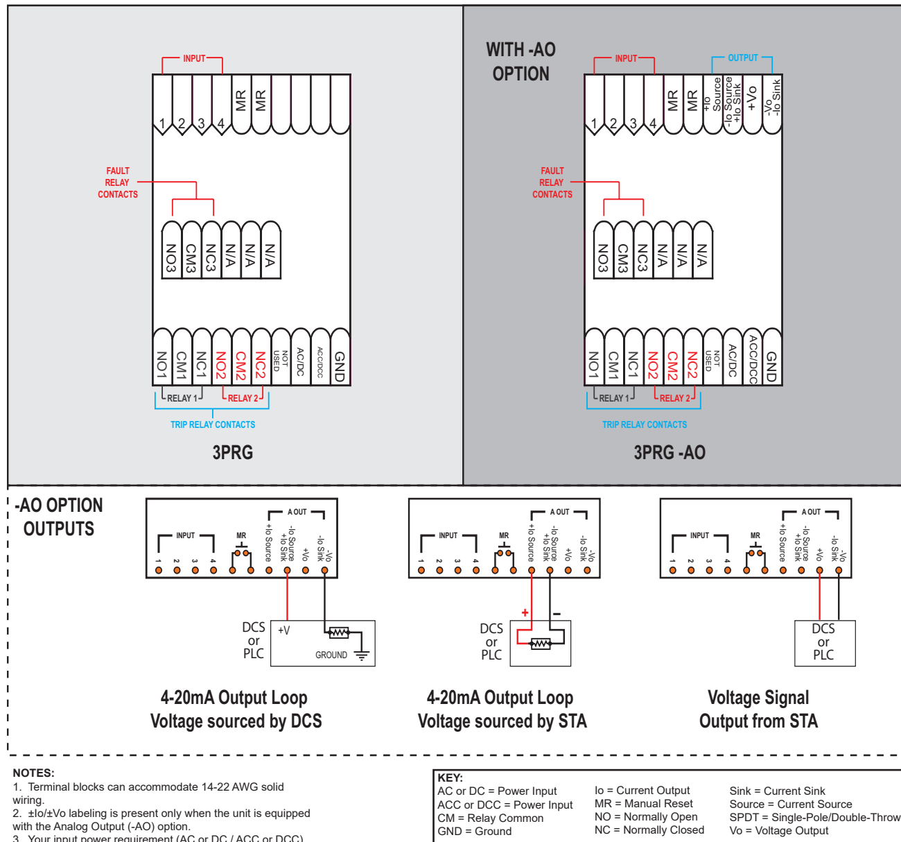
Figure 11. Terminal Designations (TPRG)
