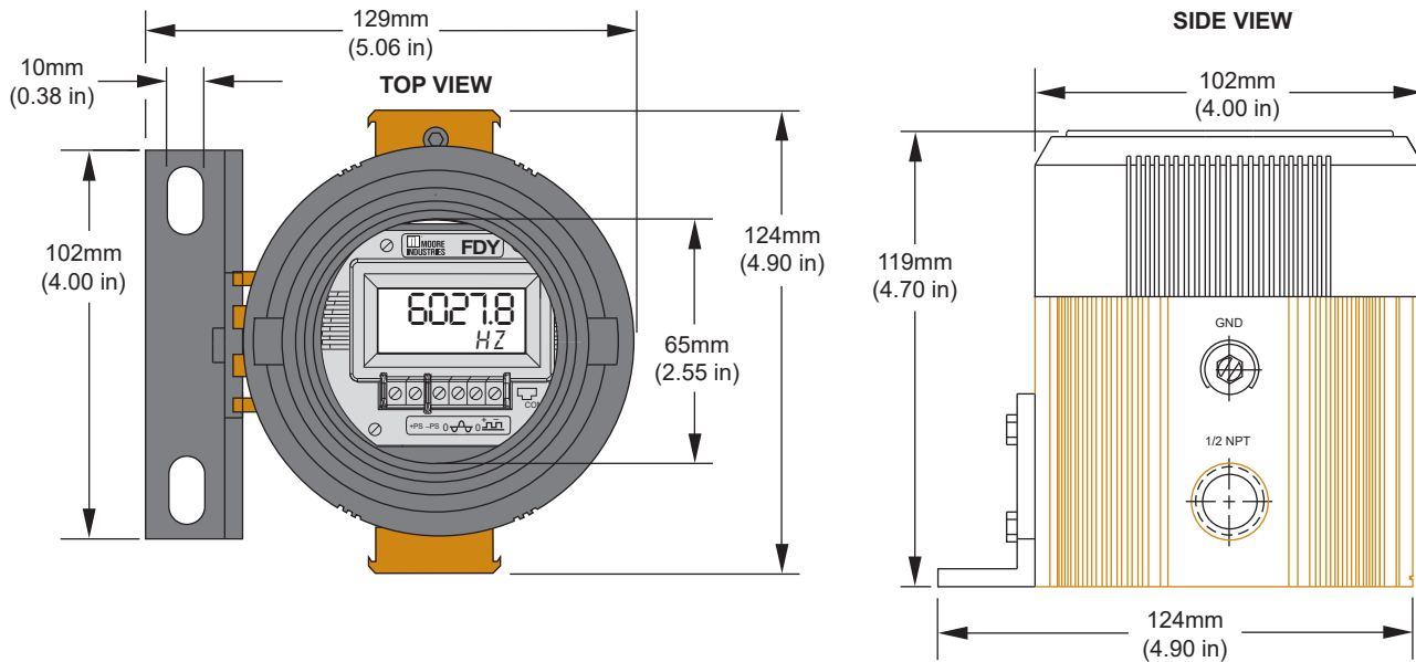
Figure 9. D-BOX Enclosure Dimensions
