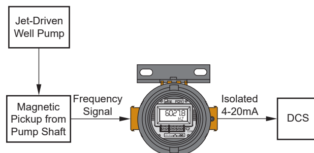
Figure 4. Monitor pump speed to ensure optimum efficiency
