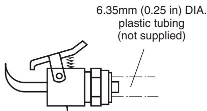
Figure 3. Test Coupler (P/N 163-202-00) for units with pneumatic test jack
