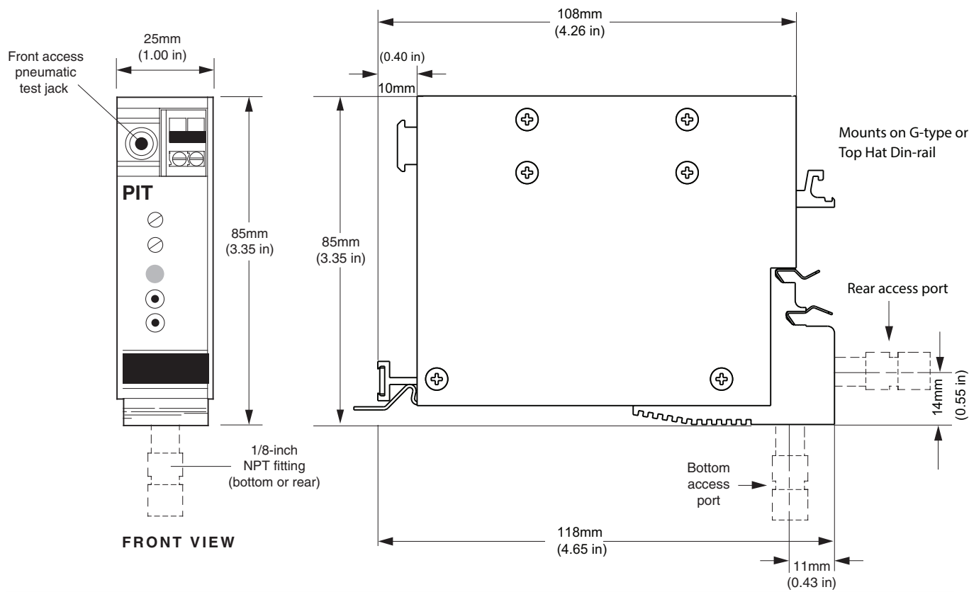
Figure 2. PIT DIN-Style Housing Dimensions
