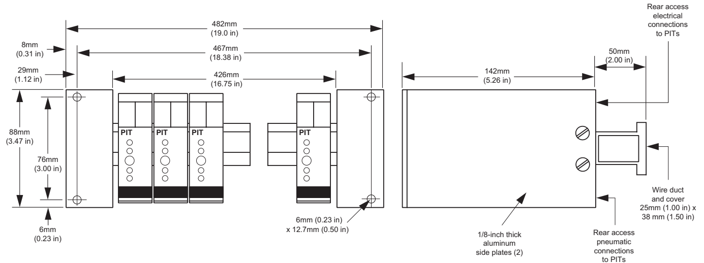
Figure 5. EXI and EXIM Housing Dimensions
